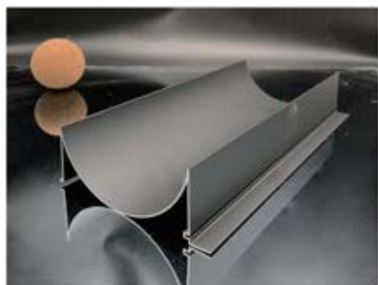
Arc Series -B43 规格size6000*100*43.2mm
