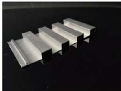
长城板系列-B09 Great Wall plate series -B09 规格size6000*120*9mm
